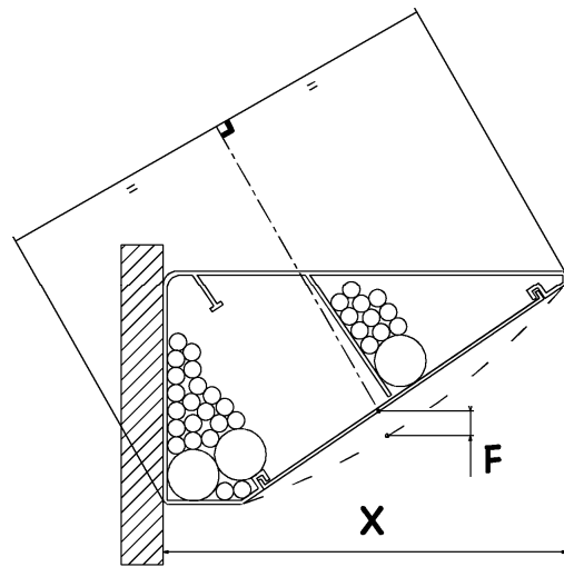
Figure 102b – SG/SCP de section transversale non rectangulaire
